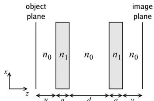
Fig. 1. Reflectionless evanescent-wave amplification (REWA) by two slab waveguides, where n_1 > n_0 .
